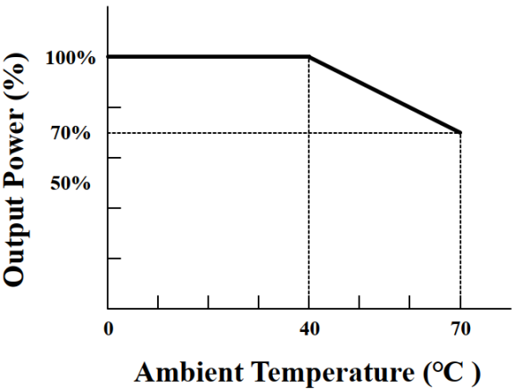
OUTPUT POWER DERATING CURVE
